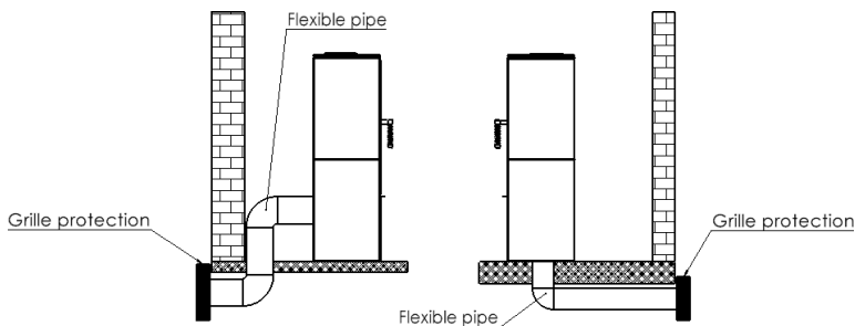
Fig. 2. Diagram of the air supply connection
