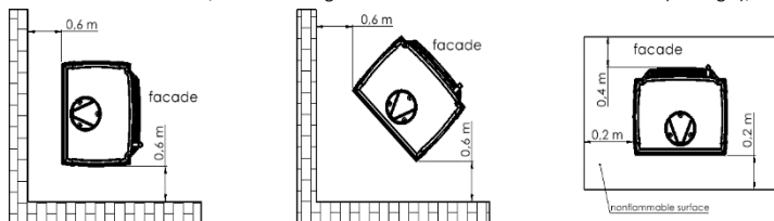
Fig.3. Safe distance from the stove
