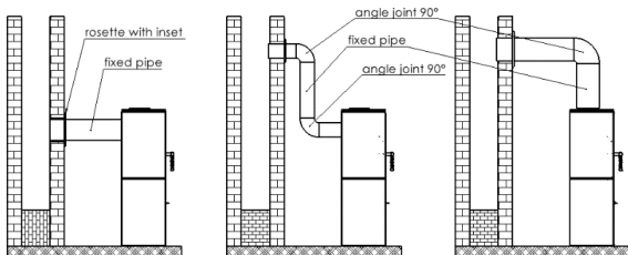
Fig.4. Schematics of fireplace stove connection
